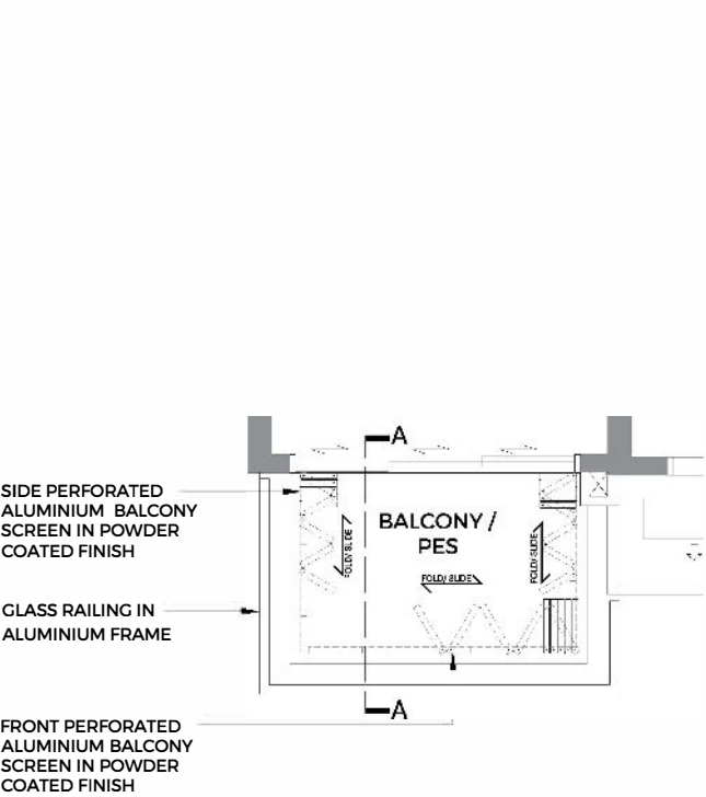
TYPICAL BALCONY / PES PLAN
